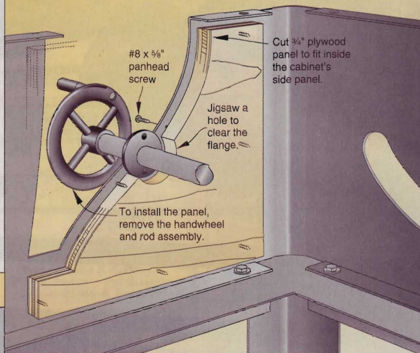
Older Craftsman saw (viewed from inside, trunion not shown)
